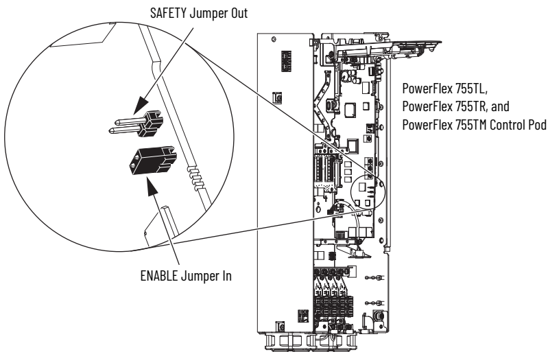
Figure 4 - PowerFlex 755T Products Jumper Locations
