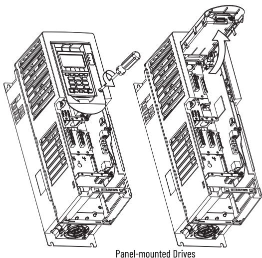
Panel-mounted Drives
