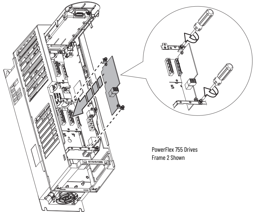
Figure 4 - Tighten Screws
